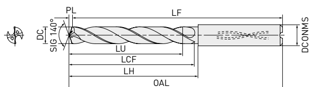
1 Cylindrical shank type
